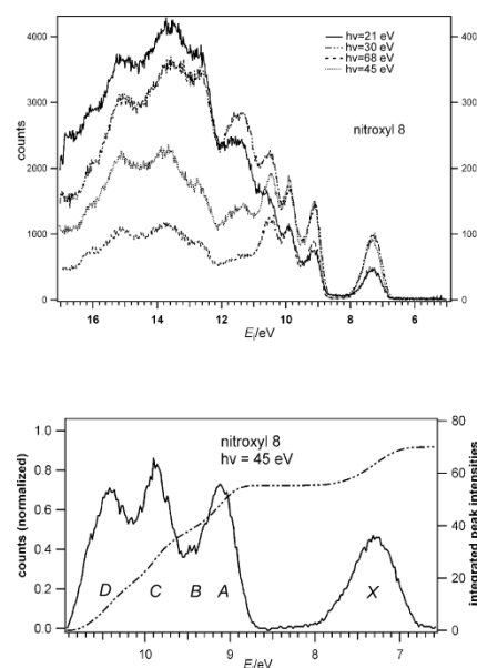
Fig.2 UV photoelectron spectra of nitroxyl8 measured at different photon energies (top panel). In the bottom panel, the dashed-dotted line gives the integrated spectral intensity in the displayed region. Spectrum measured at h\nu=45 eV is shown as an example. The intensity was normalized by dividing with max value, the fitting baseline chosen for subtraction was of ExpDec2 type.
