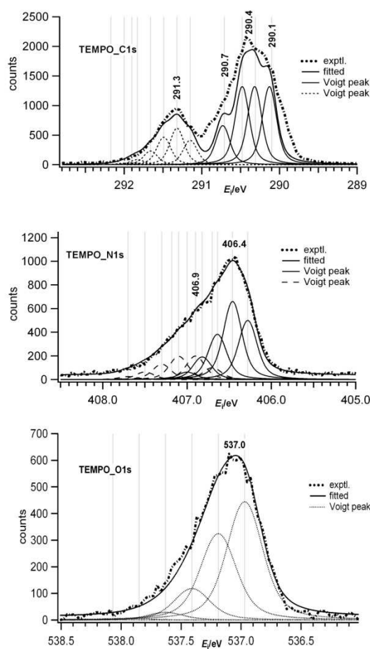
Fig. 5 C1s, N1s and O1s in XPS of TEMPO radical
