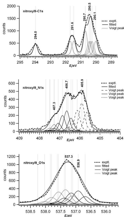
Fig. 7 C1s, N1s and O1s in XPS of nitroxyl9 radical
