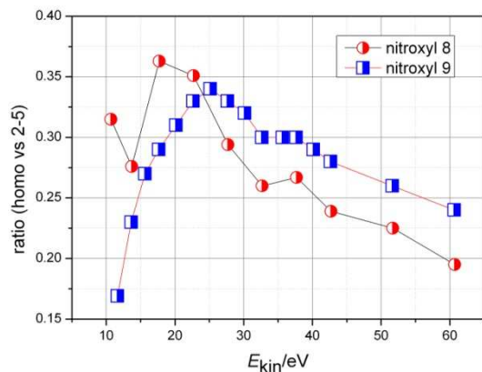
Fig. 4 Variation of relative band intensities of valence ionizations for nitroxyl8 and nitroxyl9 as a function of photoelectron kinetic energy. Ratio (homo vs 2-5) represents the ratio of intensity of the X ionization band vs. the total intensity of the subsequent four ionization bands A-D at a given photoelectron energy.
