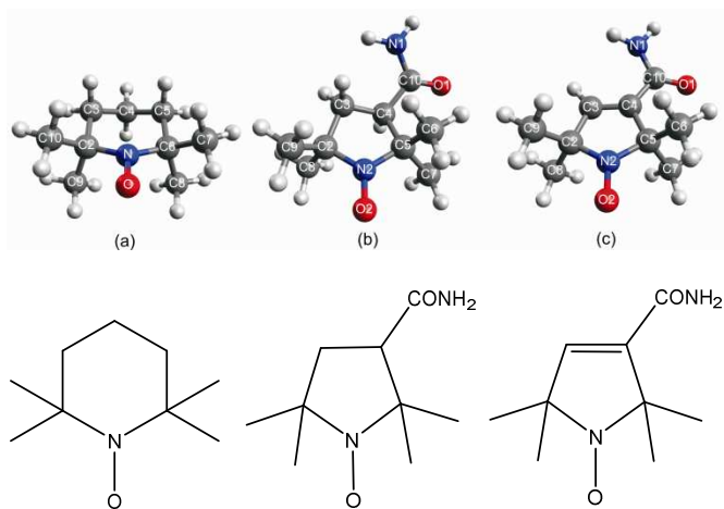
Fig. 1 Structures and labeling of the atoms of the three studied nitroxyl radicals: (a) TEMPO (C 3 symmetry) (b) nitroxyl8 and (c) nitroxyl9.
