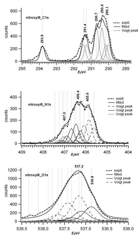
Fig. 6 C1s, N1s, O1s in XPS of nitroxyl8 radical
