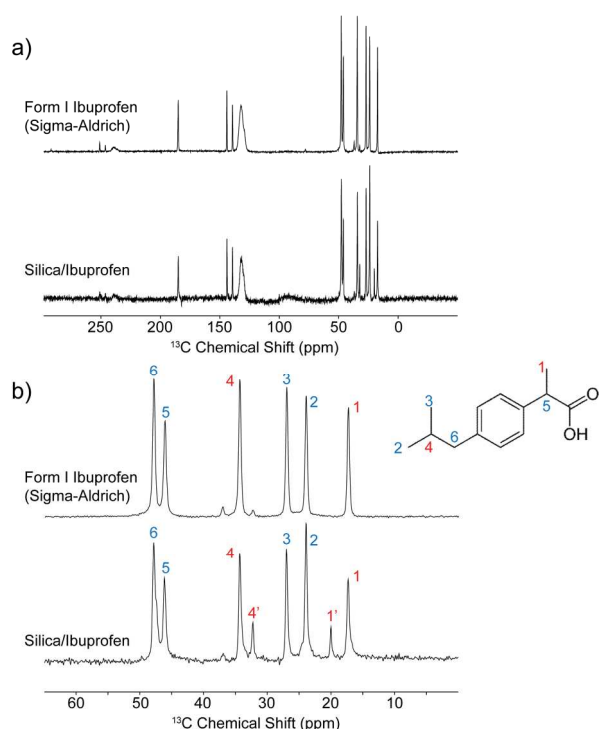
Figure 5. ^{13}\text{C} CPMAS spectra of form I IBP and silica-IBP, a) full spectra and b) expanded spectra (with ^{13}\text{C} - \delta_{\text{iso}} /ppm assignment) of the aliphatic carbon region, which clearly shows the onset of additional peaks for silica-IBP (peak 1' and 4'). The ratio of the two forms is 79:21 (Form I:unknown form).
