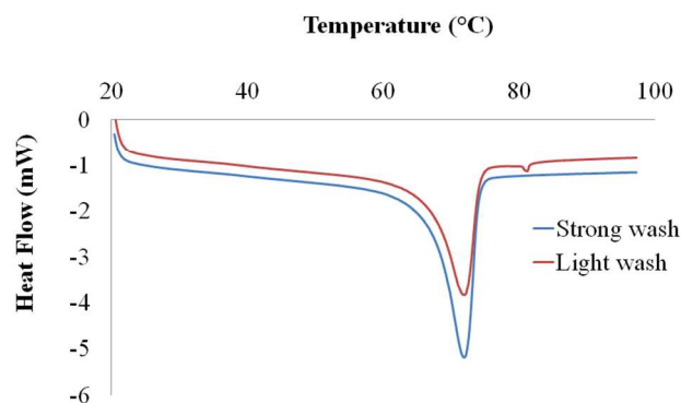
Figure 4. DSC results of FEN loaded in porous silica particles of ~40 nm pores of light- (red) and strong-wash (blue). Samples of light wash show two peaks (71.4 and 81.2 °C) while samples of strong wash has only one peak of 71.7 °C.
