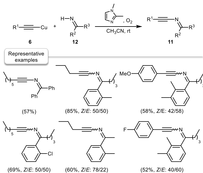
Figure 5 Click alkynylation of imines with copper acetylides for the synthesis of ynimines. Standard conditions: 2 mmol 6 , 8 mmol 12 , 4 mmol DMI, 1 atm. O 2 , 8 mL of CH 3 CN, rt, 12 h.
