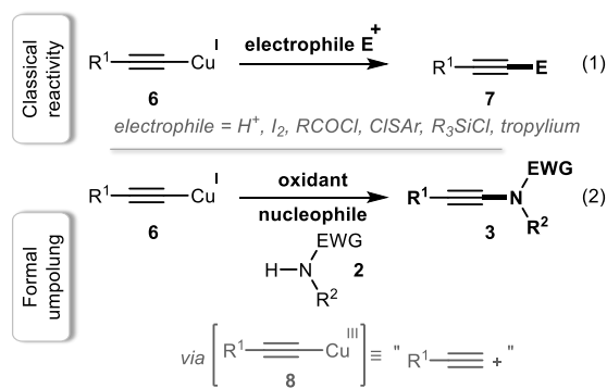
Scheme 2 Strategy: oxidative umpolung of copper acetylides.
