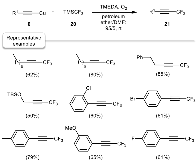
Figure 8 Oxidative alkylation of the Ruppert-Prakash reagent: direct entry to trifluoromethylated alkynes. Standard conditions: 0.5 mmol 6 , 2 mmol 20 , 0.5 mmol TMEDA, 1 atm. O 2 , 0.1 mL DMF, 1.9 mL pet. ether, rt, 24 h.
