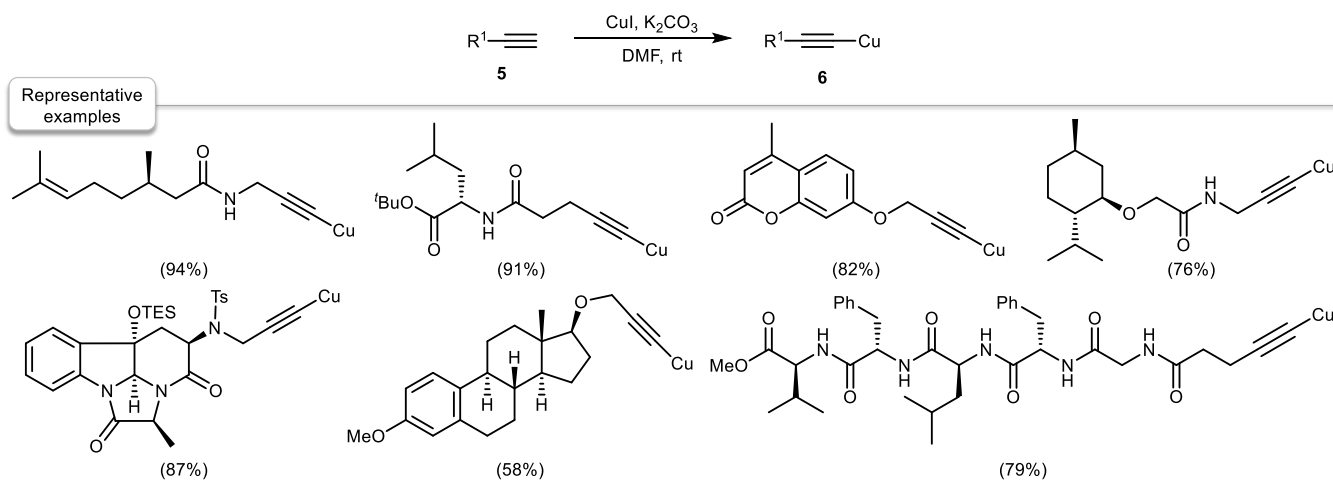
Figure 2 Synthesis of more complex copper acetylides.
