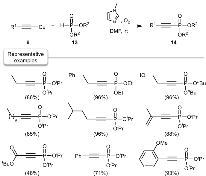
Figure 6 Oxidative alkynylation of dialkylphosphites: a practical entry to alkynylphosphonates. Standard conditions: 2 mmol 6 , 8 mmol 13 , 4 mmol NMI, 1 atm. O 2 , 4 mL of DMF, rt, 1-12 h.
