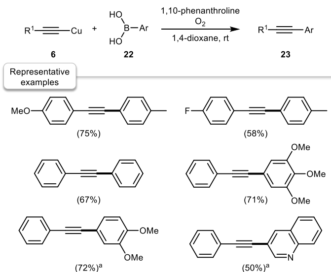
Figure 9 Expanding the scope of the oxidative alkynylation with copper acetylides: facile alkynylation of arylboronic acids (bonds formed shown in bold). a Using a 1:1 mixture of MeOH and 2,6-lutidine instead of 1,4-dioxane. Standard conditions: 0.5 mmol 6 , 1 mmol 22 , 0.5 mmol 1,10-phenanthroline, 1 atm. O 2 , 2 mL of 1,4-dioxane, rt, 48–72 h.
