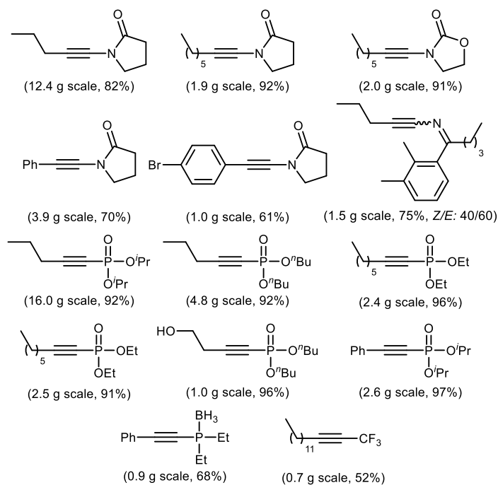
Figure 10 Gram scale alkynylation.
