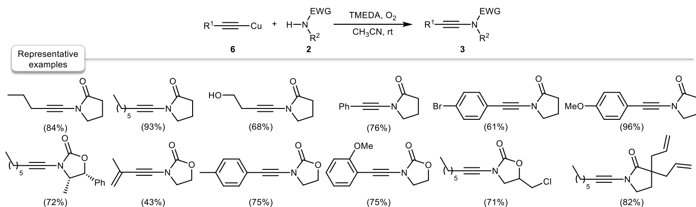
Figure 3 Facile synthesis of ynamides by oxidative alkylation of nitrogen nucleophiles with copper acetylides: a mix-and-stir reaction. Standard conditions: 2 mmol 6 , 8 mmol 2 , 2 mmol TMEDA, 1 atm. O 2 , 4 mL of CH 3 CN, rt, 24-48 h.
