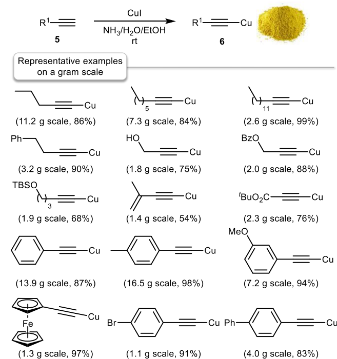
Figure 1 Synthesis of copper acetylides and representative examples prepared on a gram scale.
