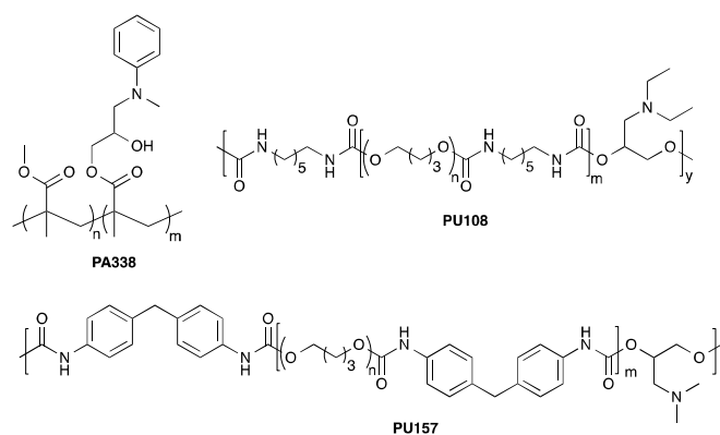
Fig 3. Structures of the copolymers PU157 , PU108 and PA338 . PU157 was synthesised from poly(butylene glycol) (mw 250) and 4,4'-methylendiphenyldiisocyanate with 3-(dimethylamino)-1,2-propanediol as an extender, PU108 from poly(butylene glycol) (mw 1000) and hexamethylenediisocyanate with 3-(diethylamino)-1,2-propanediol as an extender. PA338 is N -methyl aniline modified poly(methyl methacrylate-co-glycidyl methacrylate) (synthesised in 1:1 monomer ratio).
