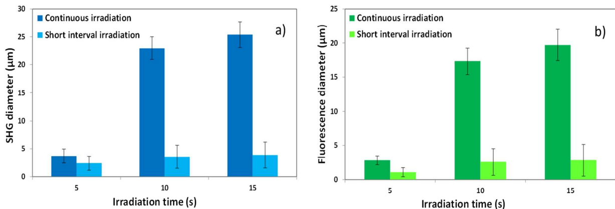
Fig.3 SHG diameter (a) and fluorescence diameter (b) as a function of laser irradiation time showing the effects of continuous and short interval irradiation with ~198 mW laser power and 800 nm irradiation (resonance) wavelength.
