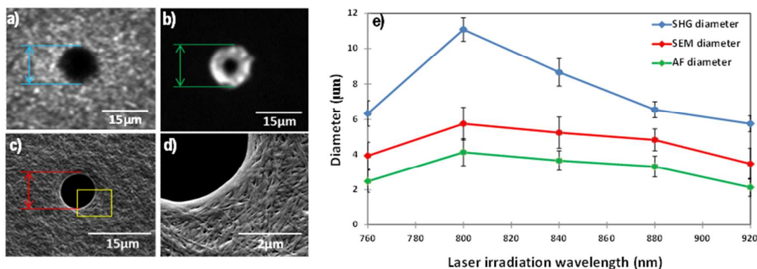
Fig.1 SHG image (a), AF image (b), SEM image of the laser induced cavity (c) obtained at the resonance wavelength (800 nm), and magnified SEM image (d, highlighted area in c) showing the banding periodicity along the border of the cavity and surrounding areas of the laser irradiated site. SHG, SEM, AF cavity sizes for different irradiation wavelengths, \sim 198 mW average laser output power and 10 s irradiation time (e).
