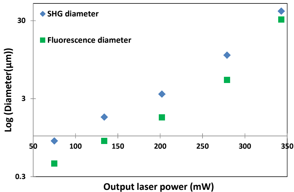
Fig.2 SHG diameter and AF diameter with varying laser output power on logarithmic scale showing exponential growth in cavity size observed at 800 nm irradiation (resonance) wavelength and 10 s irradiation time.
