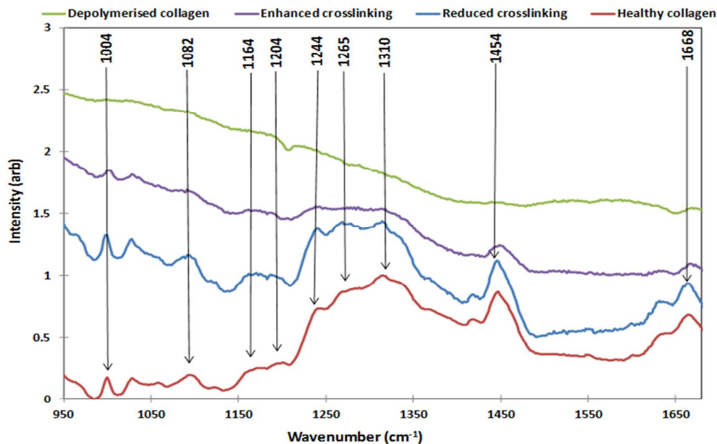
Fig.6 Raman spectra showing comparison between cluster 1 (Depolymerised collagen), cluster 2 attributing to enhanced crosslinking zone, cluster 3 representing the reduced crosslinking zone and cluster 4 classified as healthy collagen.
