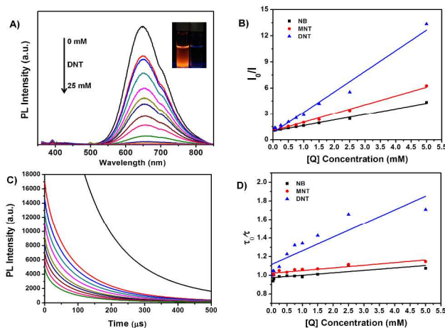
Fig.1 (A) Fluorescence quenching spectra of Si-NCs by increasing concentrations of DNT in solution with an inset showing the quenching effect with 0 and 25 mM DNT atop bench-top UV-lamp. (B) and (D) The Stern-Volmer plots for the quenching efficiencies and PL lifetimes of NB, MNT and DNT at different concentrations. (C) The PL lifetime decays of Si-NCs with increasing concentrations of DNT. The quencher concentrations for all studies can be found in Table S1†.
