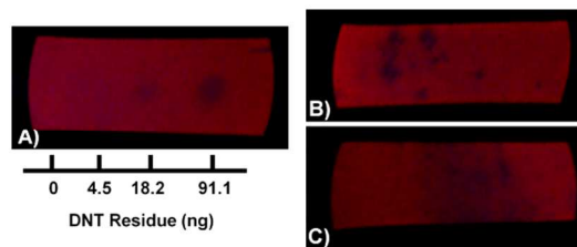
Fig. 3 Solid DNT residue testing onto Si-NCs filter paper by (A) cotton swab tips having different amounts of DNT, DNT residue left after visibly brushing off 0.5 mg DNT from a (B) plastic tray and a (C) cotton fabric, respectively.
