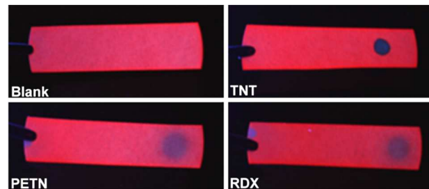
Fig. 2 Images of Si-NCs coated filter paper under a handheld UV-lamp without the presence of nitrocompound and in the presence of solutions of TNT, PETN, and RDX, as indicated.
