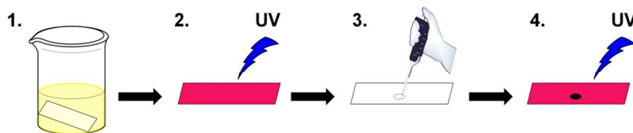
Scheme 1 Schematic representation of the preparation and use of Si-NCs based sensor paper. (1) A piece of filter paper is dip coated in a solution of concentrated Si-NCs, (2) the resulting paper is fluorescent under UV light, (3) nitroaromatic solution is spotted onto the sensing paper, (4) quenching of the spot is observed under UV light.
