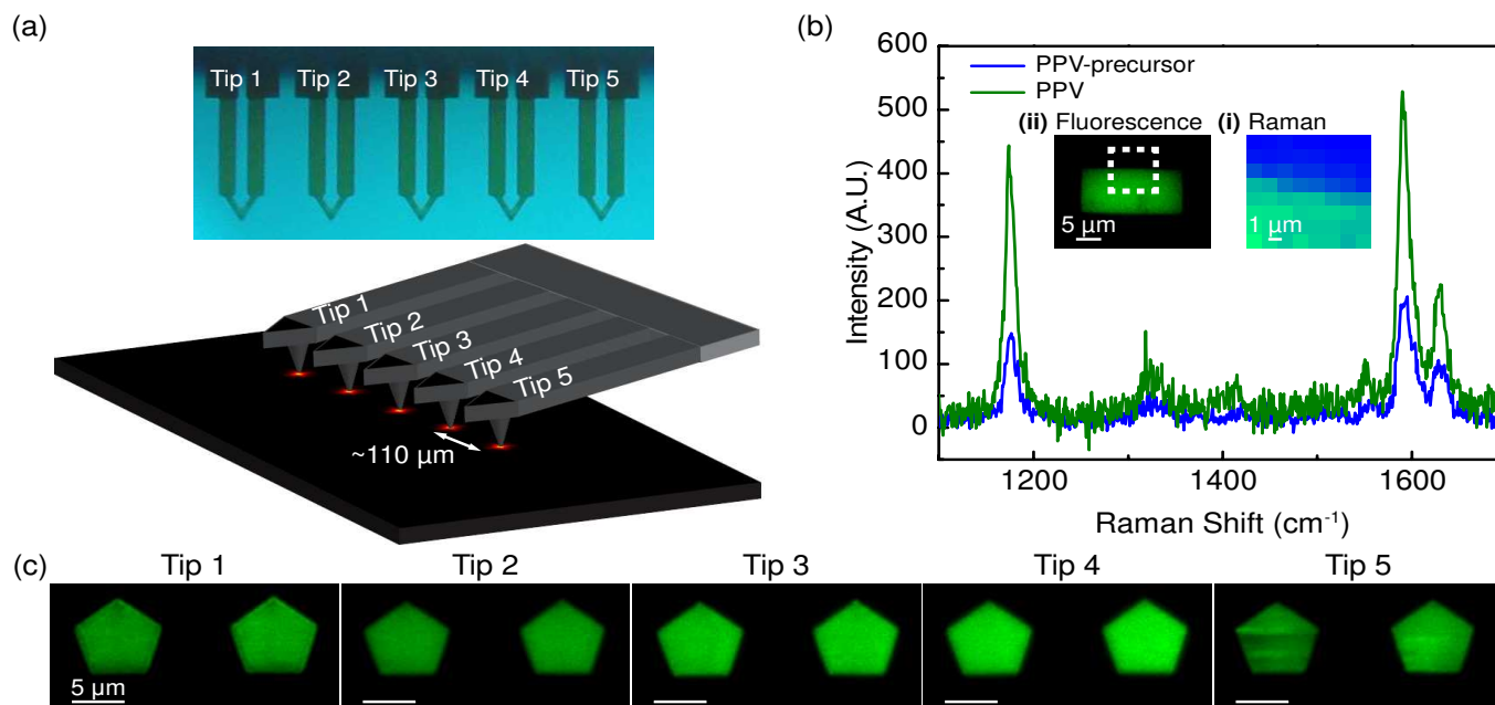
FIG. 1. (a) Optical Image and cartoon of the five thermal cantilevers and tips array for parallel TCNL. (b) Raman spectrum of PPV precursor (blue) and a TCNL produced pattern of PPV (green). In the inset we show the corresponding Raman image (I) and fluorescence image (II) of the precursor film and PPV pattern. (c) Fluorescence image of five PPV pentagonal double-patterns produced by the TCNL array and consisting each of two pentagons produced with two different temperatures.
