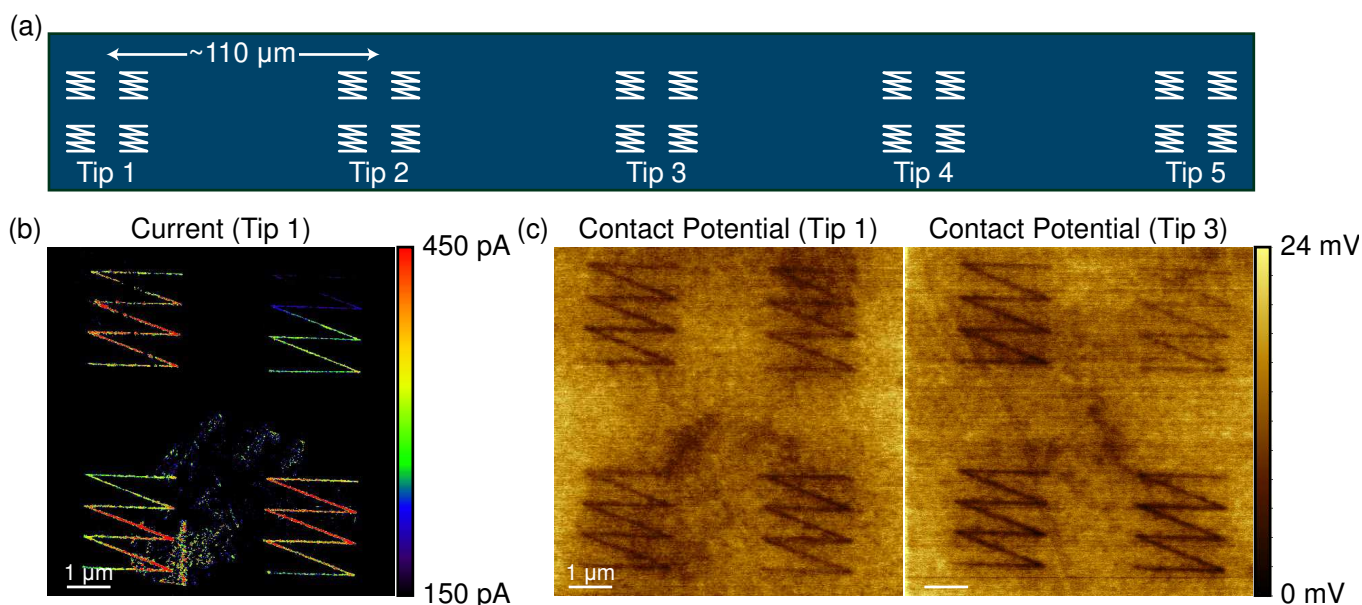
4 | Nanoscale , 2013, 00 , 1–3 FIG. 3. Parallel TCNL of reduced GO nanostructures. (a) Schematic of Parallel TCNL used to produce conductive rGO nanostructures in an insulating GO film. (b) Current and (c) Kelvin probe AFM contact potential difference for rGO nanostructures made by tip 1 and tip 3.
