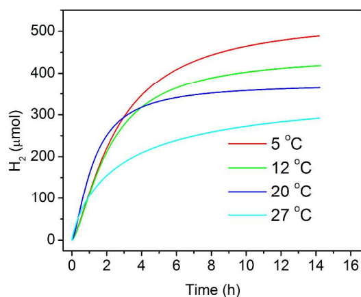
Fig. 6 Kinetics of photocatalytic hydrogen production performed at different temperatures under blue LED excitation centered at 452 nm. Conditions: 2 \times 10^{-5} M 1 , 3.3 \times 10^{-4} M [Ru(bpy) 3 ] 2+ and 0.3 M H 2 A/HA - at pH 4.
