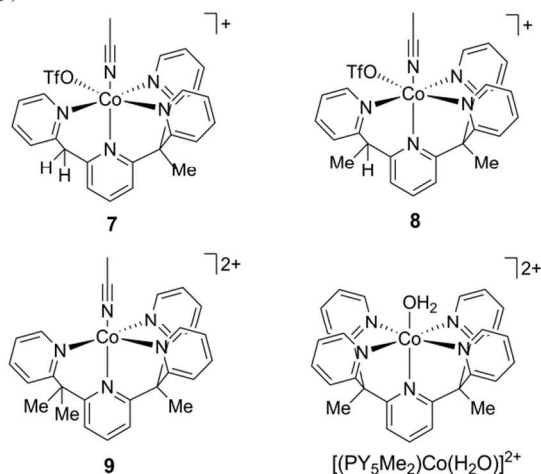
Chart 2. Tetrapyridine and pentapyridine Co 2+ catalysts (OTf = CF 3 SO 3 ).
