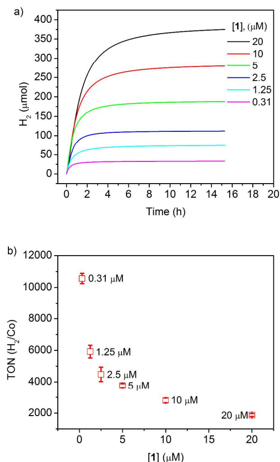
Fig. 3 (a) Hydrogen production as a function of time at different concentrations of 1 under blue LED excitation centered at 452 nm. (b) TONs (H 2 /Co) versus concentration of 1 in the presence of 3.3 × 10 -4 M [Ru(bpy) 3 ] 2+ in 0.3 M H 2 A/HA - , pH 4, measured under the same photolysis conditions as part (a).
