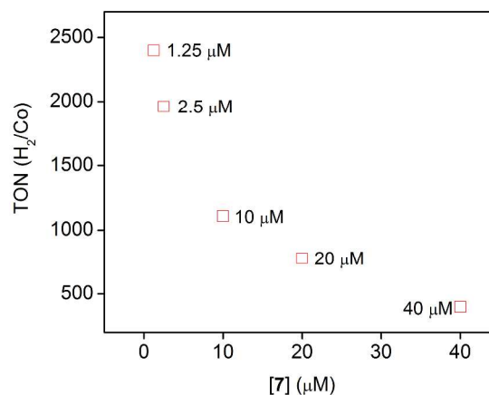
Fig. 12 TONs measured as a function of concentration of 7 in 0.3 M ascorbate in water at pH 7 containing 3.3 \times 10^{-4} M [\text{Ru}(\text{bpy})_3]\text{Cl}_2 under inert atmosphere.
