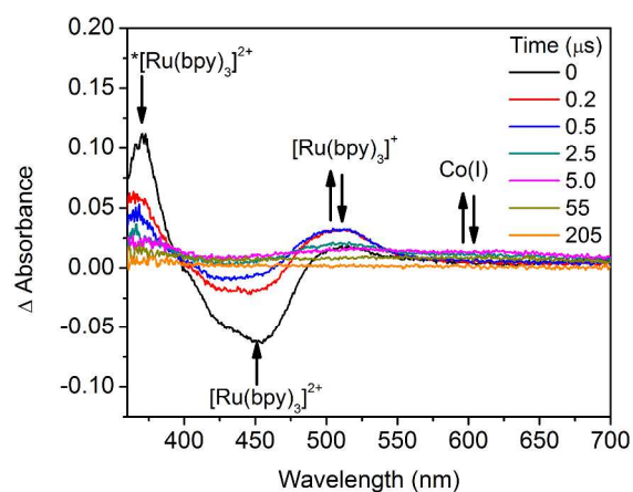
Fig. 7 Transient absorption difference spectra of a solution containing 2.9 \times 10^{-4} M 1 and 2.5 \times 10^{-5} M [Ru(bpy) 3 ] 2+ in 0.3 M H 2 A/HA - at pH 4, recorded at the specified delay times following nanosecond laser excitation at 452 nm.
