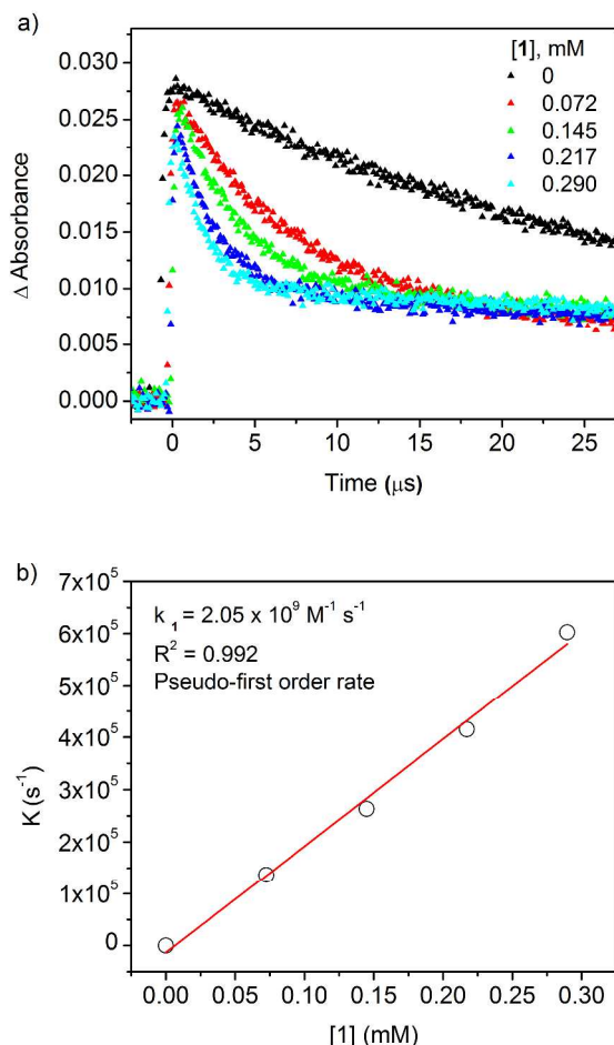
Fig. 8 (a) Absorption transients monitored at 505 nm, where both [Ru(bpy) 3 ] + and Co I (bpyPY2Me) absorb. (b) Rate of the reaction between [Ru(bpy) 3 ] + and Co II (bpyPY2Me) versus the concentration of the catalyst. Conditions: 2.5 × 10 -5 M [Ru(bpy) 3 ] 2+ in 0.3 M H 2 A/HA - at pH 4.
