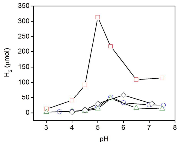
Fig. 11 Photocatalytic \text{H}_2 production in the presence of 2 \times 10^{-5} M of complex 7 (red squares), 8 (blue circles), 9 (green triangles), and [\text{CoPY5Me}_2]^{2+} (black diamonds) in a 0.3 M \text{H}_2\text{A}/\text{HA}^- aqueous solution at pH 3 to 7.5 containing 3.3 \times 10^{-4} M [\text{Ru}(\text{bpy})_3]^{2+} under an inert atmosphere.
