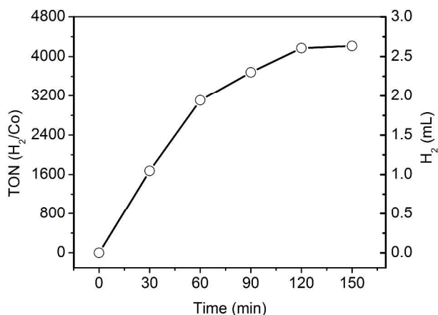
Fig. 4 Hydrogen production as a function of time observed for 25 mL of a solution containing 1 \times 10^{-6} M 1 , 3.3 \times 10^{-4} M [Ru(bpy) 3 ] 2+ and 0.3 M H 2 A/HA - at pH 4 under solar-simulated one-sun illumination (AM 1.5G, 100 mW/cm 2 ) using appropriate filters in conjunction with a Xe arc lamp.
