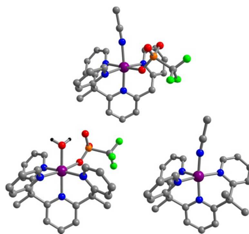
Fig. 10 Molecular structures of the mono- and dicationic Co 2+ complexes in the crystal structures of 7 (top), 8 (left), and 9 (right), respectively. Purple, blue, grey, red, orange, and green spheres represent Co, N, C, O, S, and F atoms, respectively; hydrogen atoms (other than for H 2 O in 6 ) have been omitted for clarity.
