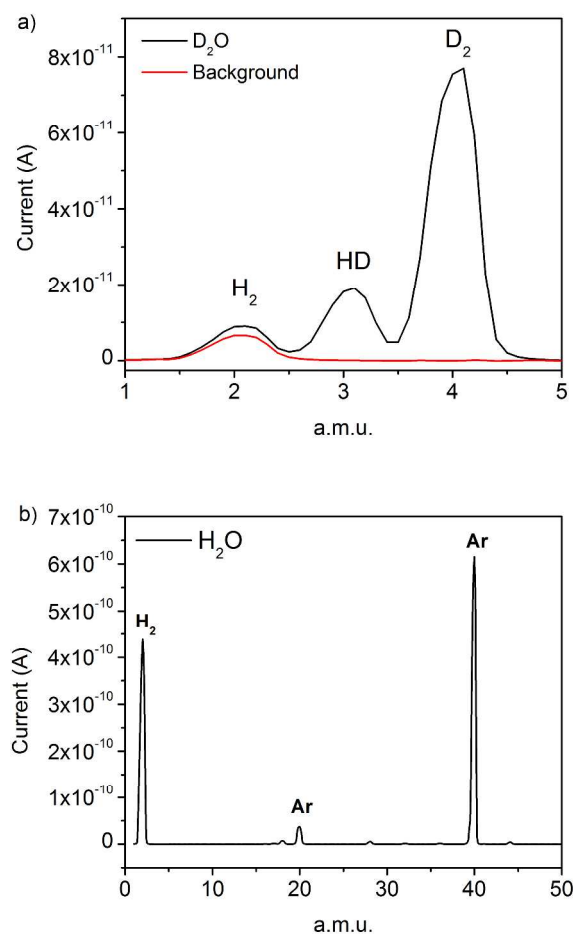
Fig. 9 (a) Mass spectrum of the analyzed headspace in the deuteration experiments (black) after photocatalysis ceases, along with the background (red) resulting from MS outgassing. The photocatalysis was induced using blue LED excitation centered at 452 nm. Conditions: 2 × 10 -5 M of 1 , 3.3 × 10 -4 M [Ru(bpy) 3 ] 2+ in 0.1 M H 2 A/HA - in D 2 O at pD = 4.0. (b) Mass spectrum of the
