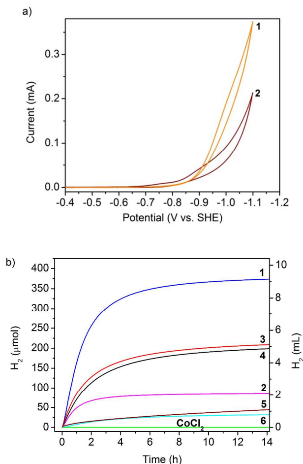
Fig. 2 (a) Cyclic voltammograms of 1 and 2 (0.2 mM) in aqueous solution containing 0.3 M H 2 A/HA - at pH 3.95 (□ = 100 mV/s) (b) Photocatalytic hydrogen production under 452 ± 10 nm (540 mW) of a solution containing 2 × 10 -5 M 1 (blue, pH 4), 2 (magenta, pH 4.5), 3 (red, pH 4.5), 4 (black, pH 4), 5 (brown, pH 5.5), 6 (light blue, pH 5.0) or CoCl 2 control (green, pH 4), 3.3 × 10 -4 M [Ru(bpy) 3 ] 2+ in 0.3 M H 2 A/HA - .
