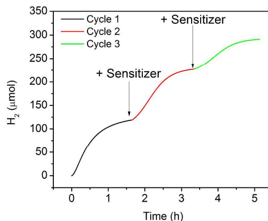
Fig. 5 Regeneration of photocatalytic hydrogen production resulting from the addition of fresh aliquots of [Ru(bpy) 3 ] 2+ . Photocatalysis was induced using blue LED excitation centered at 452 nm. Conditions: 2 \times 10^{-5} M 1 , 2 \times 10^{-5} M [Ru(bpy) 3 ] 2+ and 0.3 M H 2 A/HA - at pH 4.
