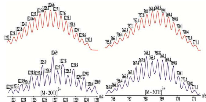
Figure 1. Theoretical (red, top) and experimental (blue, bottom) ESI-MS regions corresponding to [3 - 2OTf]^{2+} (left) and [3 - 3OTf]^{3+} (right) charge states of 3 .
