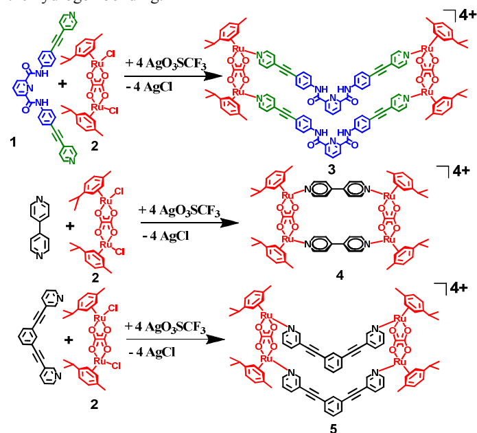
Scheme 2. Synthesis of metallacycles 3-5
