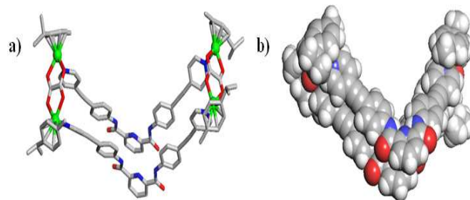
Figure 2. (a) The structure of 3 reveals a [2 + 2] assembly. (b) Space filling model of 3 .
