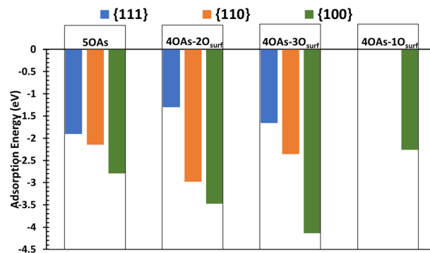
Fig. 1 Adsorption energies of arsenate species in different binding configurations on the stoichiometric \{111\} , \{110\} , and \{100\} surfaces of \text{CeO}_2 . 5OAs denotes five-fold coordinated As species, and 4OAs-1O surf , 4OAs-2O surf , 4OAs-3O surf denote four-fold coordinated As species adsorbed in monodentate, bidentate and tridentate configurations, respectively.
