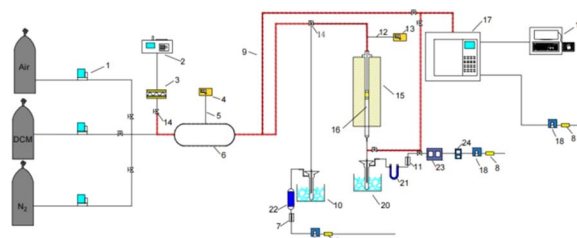
Fig. 2 Catalyst activity evaluation device diagram. (1) Mass flow meter; (2) syringe pump; (3) carburetor; (4) temperature controller; (5) thermocouples; (6) static mixer; (7) rotor flowmeter; (8) activated carbon adsorption tube; (9) heating belt with heat tracing insulation; (10) cold trap; (11) rotor flowmeter; (12) thermocouples; (13) temperature controller; (14) valves; (15) heating furnace; (16) quartz tube; (17) gas chromatograph; (18) peristaltic pump; (19) computer; (20) cold trap; (21) U tube; (22) drier tube; (23) CO 2 detector and CO detector; (24) chlorine gas detector.
