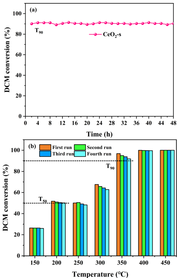
Fig. 12 Stability performance test of \text{CeO}_2\text{-s} catalyst for DCM catalytic oxidation (a), durability test of \text{CeO}_2\text{-s} catalyst for DCM catalytic oxidation at 150\text{--}450^\circ\text{C} (b).
