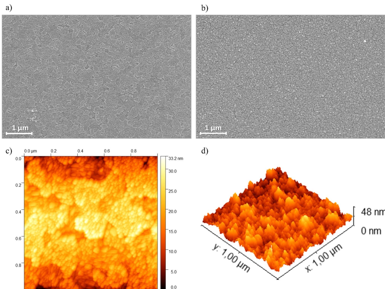
Fig. 6 SEM images of (a) bare ITO and (b) PEDOT-TPPF 16 film. Scale bars are 1 μm. (c) AFM images of ITO electrode surface (scan size 1 × 1 μm) registered after electrodeposition of porphyrin film. (d) Three-dimensional representation of the electrode surfaces measured by AFM. Films were grown cycling in the same conditions of the exhibited in Fig. 3.
