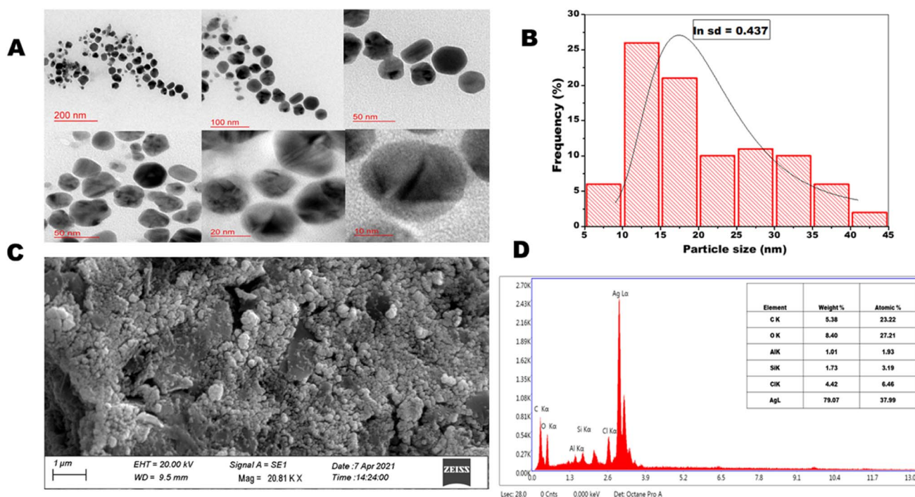
Fig. 2 (A) HRTEM images at scale bar 200, 100, 50, 20, and 10 nm, spherical silver nanoparticles of OSaAgNPs. (B) Size distribution histogram of OSaAgNPs. (C) SEM image of green synthesized OSaAgNPs. (D) Energy dispersive X-ray spectrum and chemical composition of OSaAgNPs.
