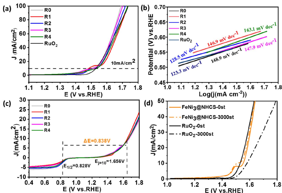
Fig. 7 (a) LSV curves of RuO 2 and samples (R0–R4) in O 2 -saturated 1 M KOH at scan rate of 5 mV s -1 at 1600 rpm and (b) Tafel plots; (c) over all LSV curves in O 2 -saturated 0.1 M KOH of sample (R0–R4); (d) LSV curves of RuO 2 and sample R2 before and after stability test.
