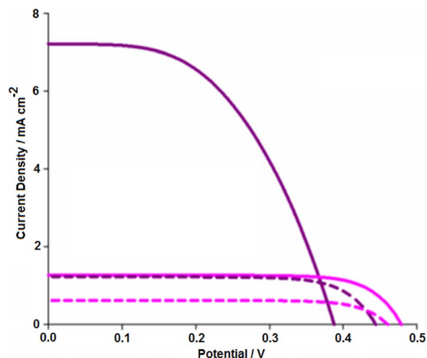
Fig. 6 Plot of current density against voltage for illuminated devices containing both AY1 (pink) and AY1 plus citric acid (purple) under full illumination (solid lines) and 10% illumination (dashed lines).
