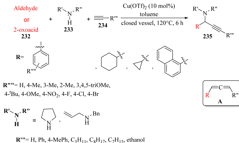
Scheme 97 Cu(OTf) 2 -catalyzed synthesis of propargylamine derivatives. 100
