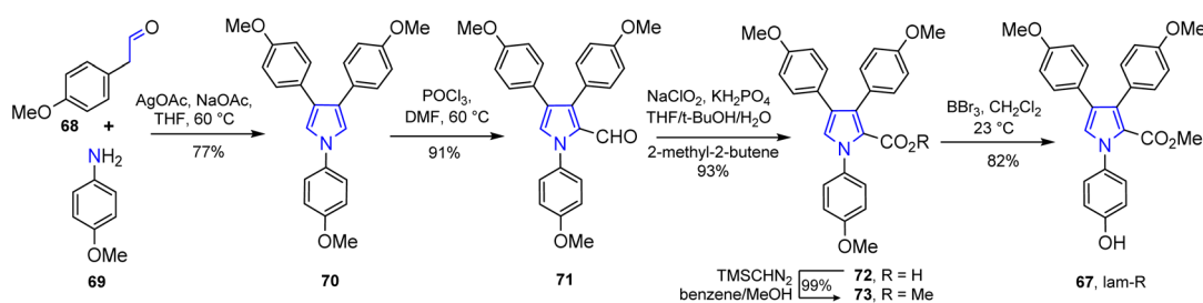
Scheme 3 Total synthesis of lamellarin R (67).
