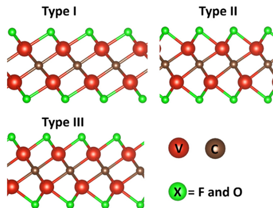
Fig. 1 Three possible binding sites for surface functionalization on V 2 CT 2 MXenes.
