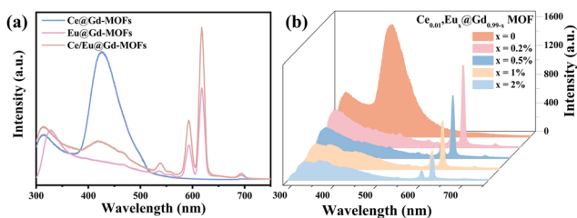
Fig. 2 (a) Emission spectra of Ce@Gd-MOFs, Eu@Gd-MOFs and Ce/Eu@Gd-MOFs, and (b) emission spectra of Ce/Eu@Gd-MOFs ( \lambda_{\text{ex}} = 260 nm).
