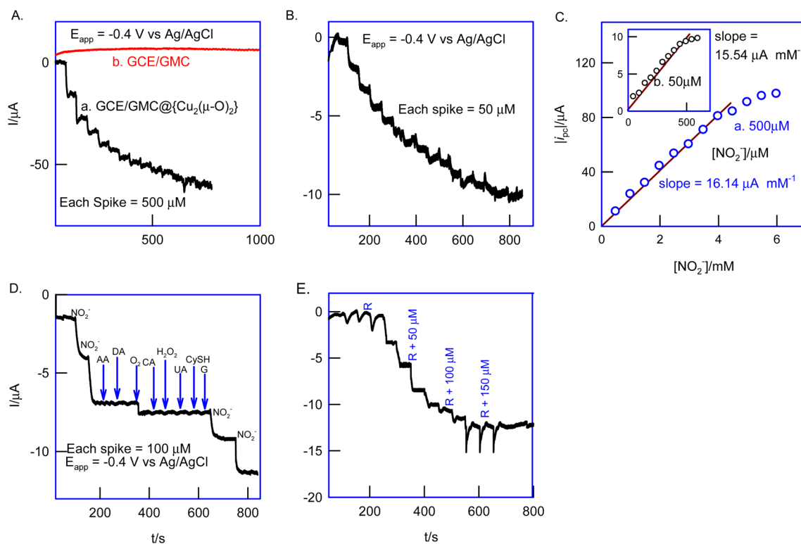
Fig. 12 Comparative amperometric i-t responses of GCE/GMC@{Cu 2 (μ-O) 2 with continuous spikes of (A) 500 μM (curve b is the control response of the GCE/GMC) and (B) 50 μM NO 2 - ; (C) calibration plots of i_{pc} vs. [NO 2 - ] in different NO 2 - concentration regions. (D) Effect of interference of various analytes. (E) Analysis of a tap water sample.
