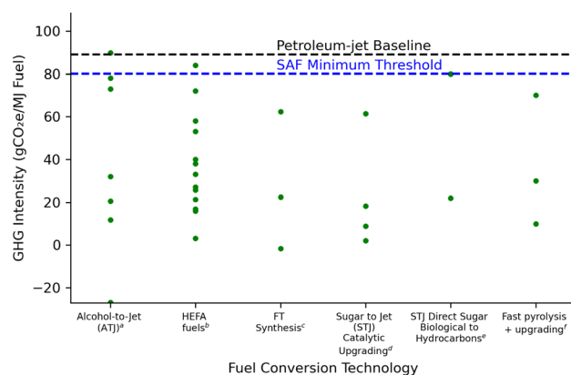
Fig. 1 GHG intensity SAF pathway comparison to fuel conversion technology pathways: ATJ, HEFA fuels, FT synthesis, and STJ catalytic.
