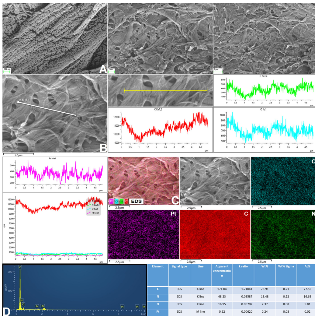
Fig. 3 SEM analysis. (A) SEM of PCMS (100 nm, 1 \mu\text{m} and 2 \mu\text{m} ). (B) Total number of distribution graphs. (C and D) EDS mapping and linear total spectrogram of PCMS (PCMS, Pt@CS/Mel@S; Mel, melatonin; CS, chitosan; S, L-serine).
