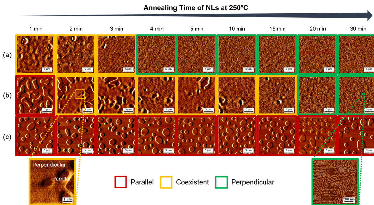
Fig. 2 AFM phase images (20 \mu m square) of PS-(OH) 2 -PMMA thin films ( \sim 30 nm) applied onto (a) P(S-r-MMA-r-HEMA) neutral layers, (b) PS-(OH) 2 -PMMA neutral layers, and (c) PS- b -PMMA neutral layers, which were annealed for various times from 1 to 30 minutes, accompanied by the magnified AFM phase images of coexistent orientation (5 \mu m square, bottom left) and perpendicular orientation (1 \mu m square, bottom right).
