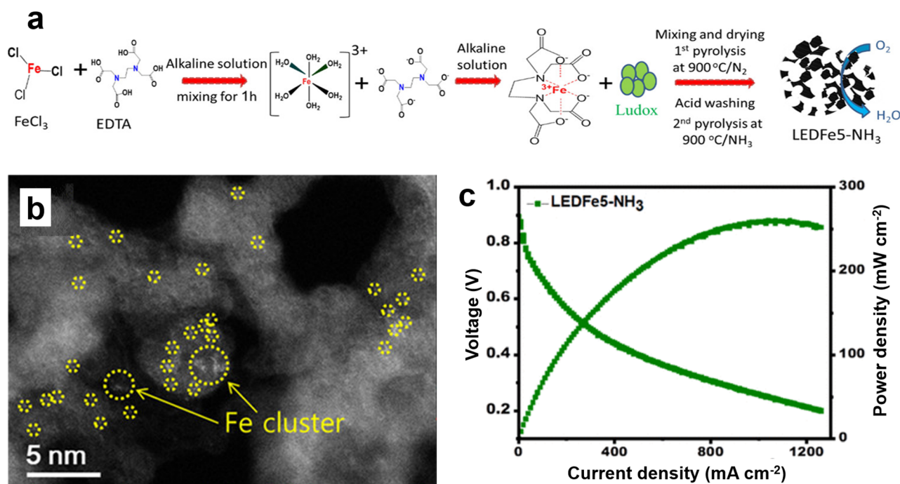
Fig. 12 (a) Schematic illustration of synthesis process for EDTA–Fe complex-based catalyst; (b) HAADF–STEM image of LEDFe 5 –NH 3 ; (c) single-cell performance of HT-PEMFC at 1.5 \text{ bar O}_2 pressure and 150 \text{ }^\circ\text{C} cell temperature. Reprinted with permission from ref. 62. Copyright 2014, American Chemical Society.
