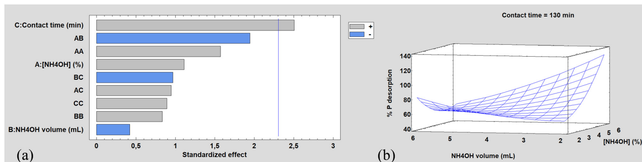
Fig. 6 CCD results: (a) standardized Pareto chart. (b) Response surface. The P desorption percentage is referred to phosphate species.
