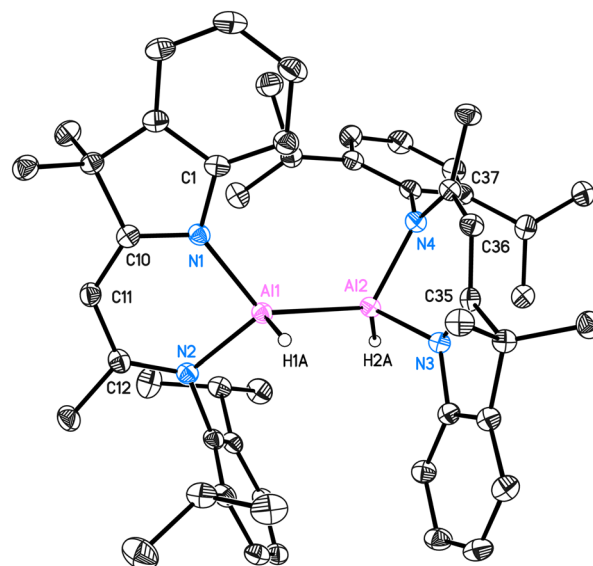
Fig. 1 Molecular structure of [(^{DNI}(H)Al)_2] ( 2 ). The anisotropic displacement parameters are depicted at 50% probability level. All ligand-based hydrogen atoms are omitted for clarity. Selected bond lengths (Å) and angles (°): Al(1)–Al(2) 2.6007(6), Al(1)–H(1A) 1.519(12), Al(2)–H(2A) 1.528(13), Al(1)–N(1) 1.9235(11), Al(1)–N(2) 1.9407(11), Al(2)–N(3) 1.9257(11), Al(2)–N(4) 1.9391(11); N(1)–Al(1)–N(2) 93.27(5), N(3)–Al(2)–N(4) 92.60(5), H(1A)–Al(1)–Al(2) 107.6(6), H(2A)–Al(2)–Al(1) 125.0(6), C(10)–C(11)–C(12) 125.64(12), C(35)–C(36)–C(37) 125.58(11).
