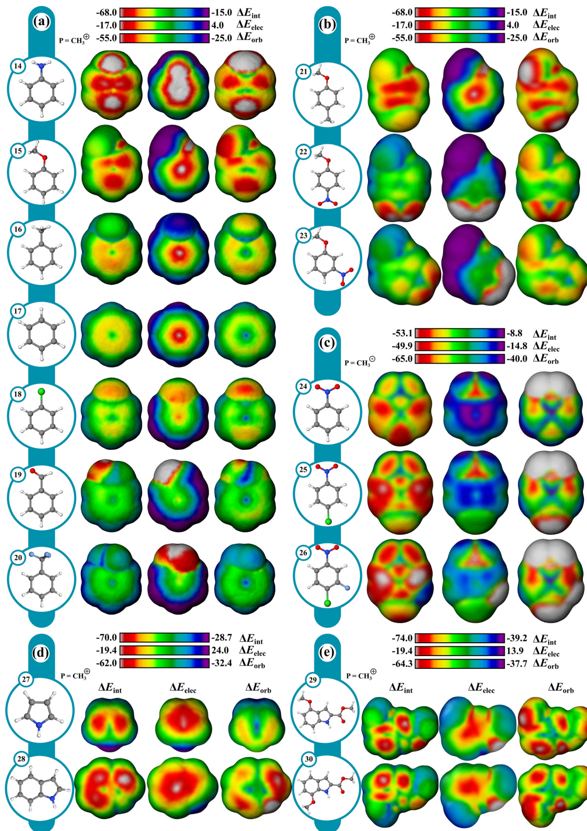
Fig. 5 From left to right \Delta E_{\text{int}} , \Delta E_{\text{elec}} , and \Delta E_{\text{orb}} IMIP's of (a) mono-, (b) di-substituted benzene derivatives (probe = CH 3 + ), and (c) surfaces generated with CH 3 - probe for benzene derivatives. Surfaces for (d) pyrrole, indole, and (e) indole derivatives (probe = CH 3 + ); isodensity: 6.00 \times 10^{-5} ; method B.
