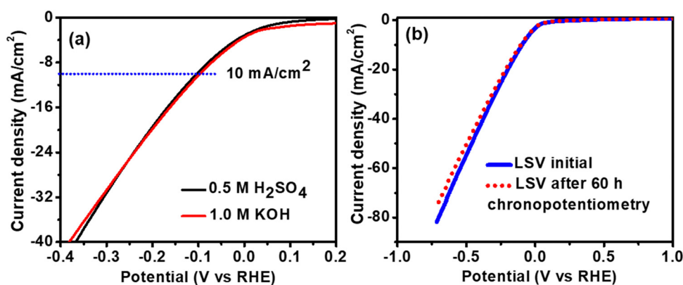
Fig. 5 (a) The LSV curves of TP-COF-C700 using 0.5 M \text{H}_2\text{SO}_4 (black line) and 1.0 M KOH (red line) electrolytes. (b) The LSV polarization curves of TP-COF-C700 before and after 60 h chronopotentiometry using 1 M KOH as electrolyte.
