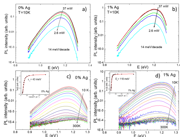
Fig. 7 The laser power (a and b) and temperature dependencies (c and d) of the PL spectra for CZCdTS monograin powders with Ag content of 0 at% and 1 at%. The inset graphs present the thermal activation energies derived from the temperature dependencies of the PL spectra. Reproduced from ref. 28 with permission from the Royal Society of Chemistry, Copyright 2019.
