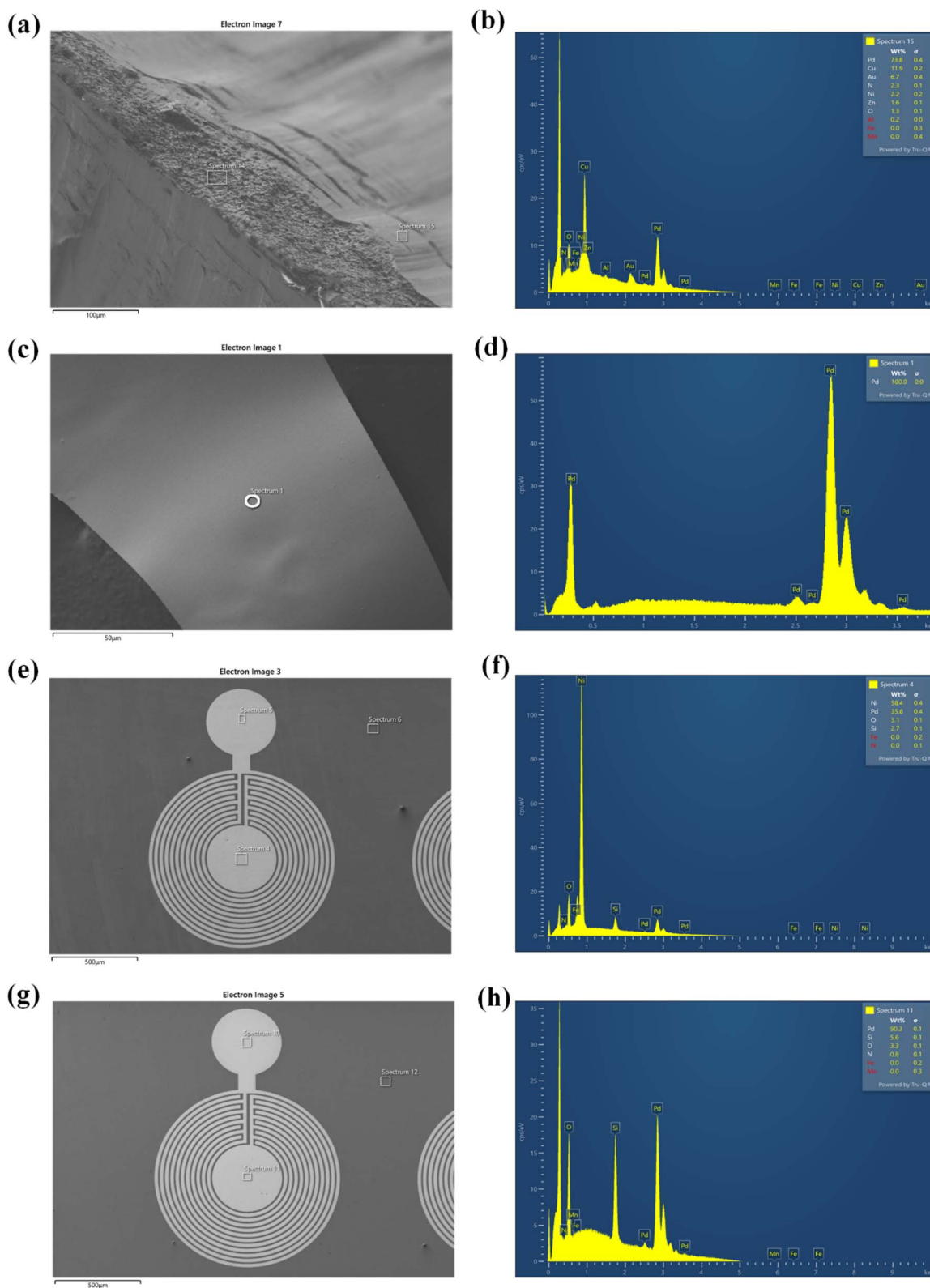
Fig. 2 SEM images and corresponding EDS spectra of (a and b) waste wires; (c and d) peeled flakes from waste wires; (e and f) e-beam evaporated electrodes from recycled Pd; (g and h) e-beam evaporated electrodes from commercial Pd.
