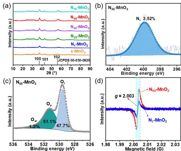
Fig. 1 (a) XRD patterns of N_y - MnO_2 ( y = 1, 25, 40, 55, 70 ) and \epsilon - MnO_2 ; (b) N 1s and (c) O 1s XPS spectra of N_{55} - MnO_2 ( O_w : oxygen from water adsorption); (d) EPR spectra of N_1 - MnO_2 and N_{55} - MnO_2 .
