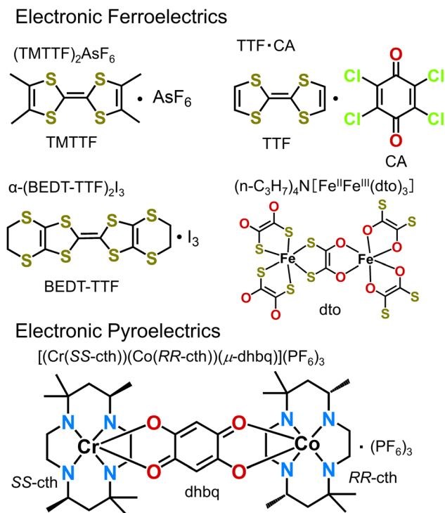
Fig. 1 Chemical structures of representative electronic ferroelectrics and electronic pyroelectrics: (TMTTF) 2 AsF 6 , α-(BEDT-TTF) 2 I 3 , TTF-CA, (n-C 3 H 7 ) 4 N[Fe II Fe III (dto) 3 ], and [(Cr(SS-cth))(Co(RR-cth))(μ-dhbq)](PF 6 ) 3 .
