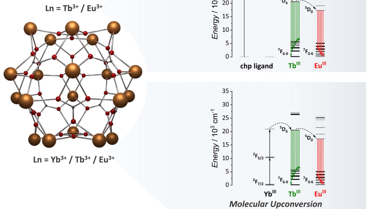
Fig. 7 Metal core structure of the {Ln 20 } MCAs (CCDC number: 2023766) 81 and the energy transfer mechanism for antenna effect and UC emissions. 81,95 Colour code: Dark orange: Ln 3+ ; grey: carbon; red: oxygen. Hydrogen atoms were omitted in the structure for clarity.
