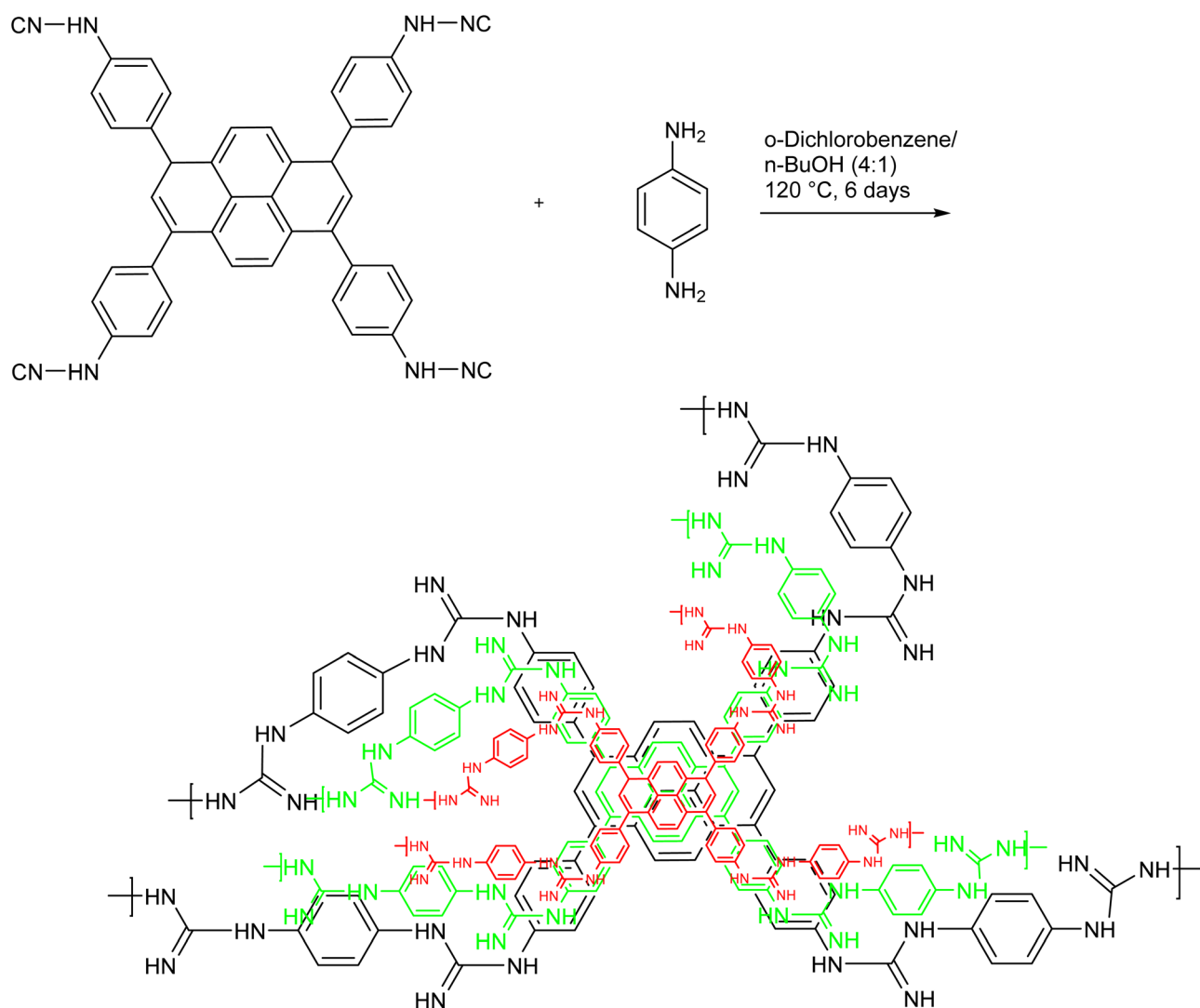
Fig. 15 The preparative process of guanidine-containing CONs. Reproduced with permission from ref. 92.
