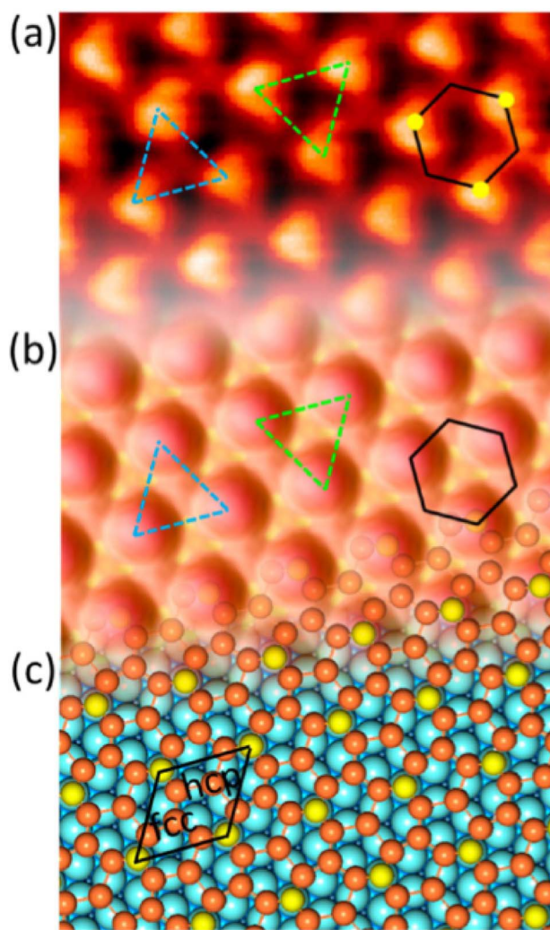
Fig. 7 Experimental (a) and simulated (b) STM images of the silicene/Ir(111) system. (c) Top view of the relaxed atomic model of the (\sqrt{3} \times \sqrt{3}) silicene/ (\sqrt{7} \times \sqrt{7}) Ir(111) configuration. Adapted with permission from ref. 16, Copyright 2013 American Chemical Society.
