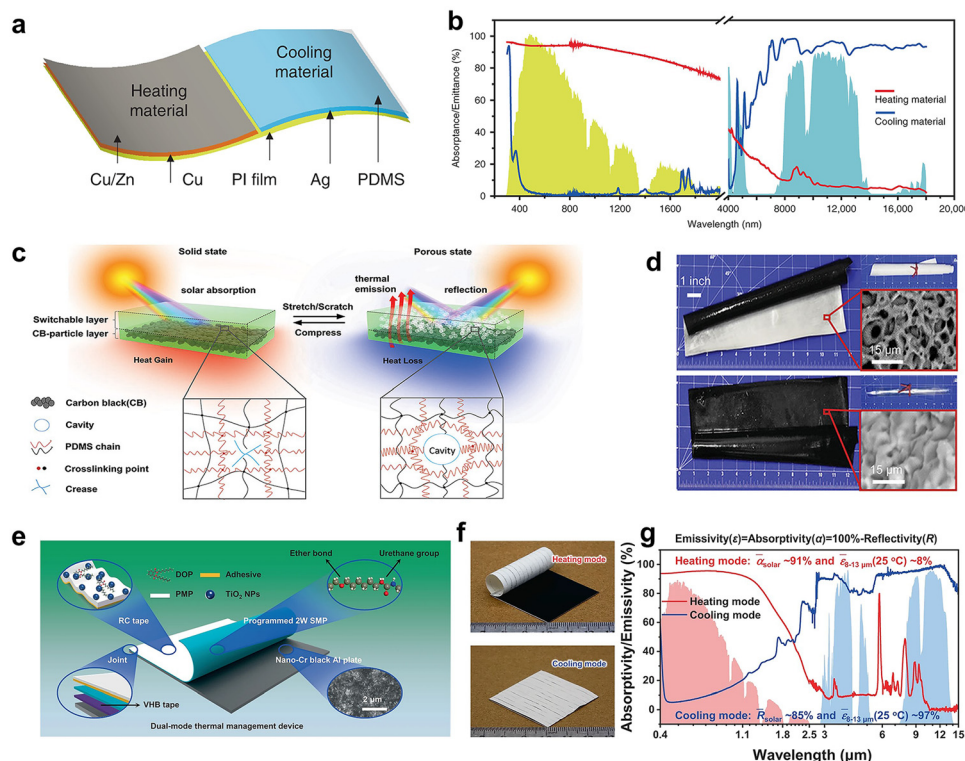
Fig. 10 (a) Structure diagram of dual-mode heating/cooling device. (b) Spectral UV-Vis-IR absorptance/emittance of the dual-mode device. Reproduced with permission from ref. 132. Copyright 2020, Nature Publishing Group. (c) Schematic illustration of the double-layer structure composed of a switchable silicon. (d) The optical photo and the SEM images of a free-standing SPDMS2.0-CBP film in porous (top) and solid (bottom) states, respectively. Insets: The SPDMS2.0 single-layer film in different states. Reproduced with permission from ref. 134. Copyright 2020, Wiley-VCH GmbH. (e) Structural diagram, (f) optical photo, (g) Spectral UV-Vis-IR absorptivity/emissivity of the dual-mode device. Reproduced with permission from ref. 135. Copyright 2022, Nature Publishing Group.
