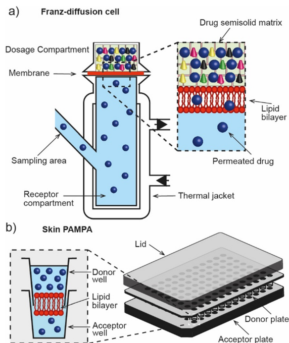
Fig. 2 In vitro dermal absorption methods. a) Franz-diffusion cell for screening the dermal absorption of chemical species across an ex vivo or synthetic membrane. b) Skin PAMPA assay for high-throughput in vitro dermal absorption screening.
