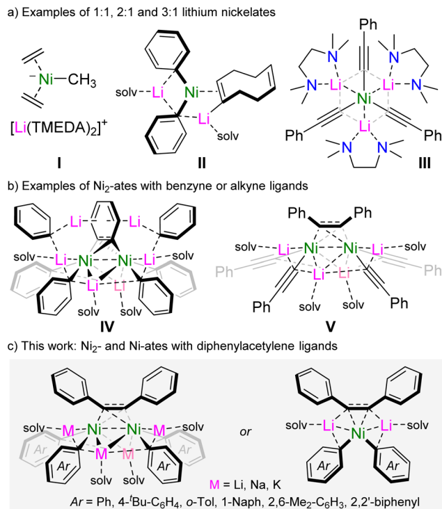
Scheme 1 Selected examples of alkali-metal nickelates.
