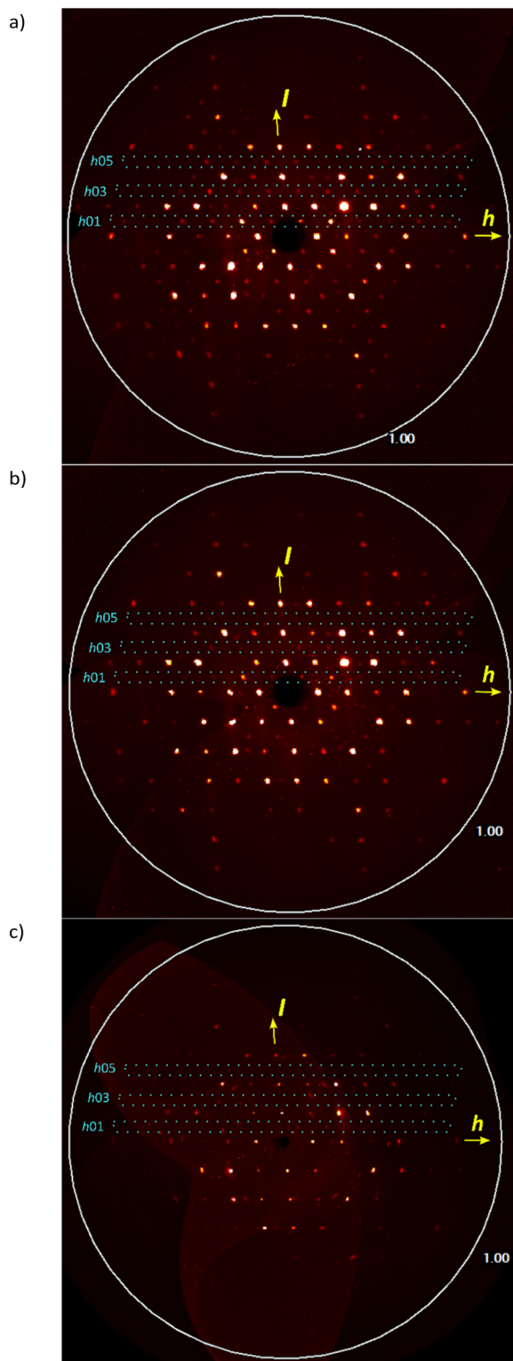
Fig. 8 Pseudo ( h 0 l ) precession images for (a) the room temperature reacted crystal at ~64% (just before transformation), and after the P\bar{1} to C2/c transformation at (b) ~79% and (c) ~89% conversion. The ( h 01), ( h 03), and ( h 05) reflections enclosed with dotted lines are allowed in the triclinic P\bar{1} space group (a) but are weaker in (b) and absent in (c) as required for C2/c .
