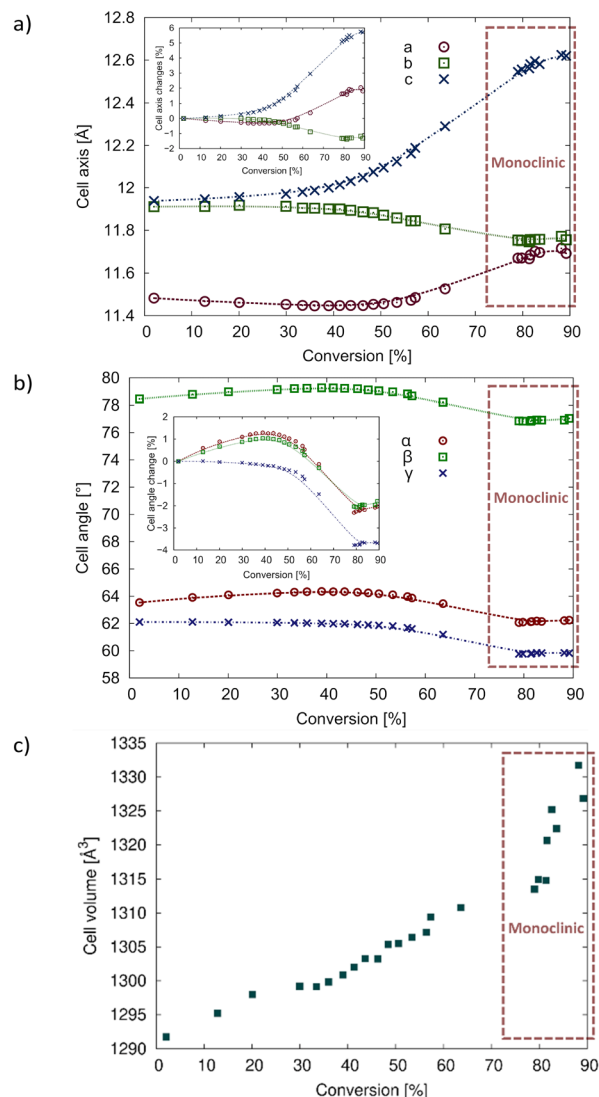
Fig. 9 Changes in unit cell parameters with degree of conversion for the crystal reacted at 20 °C. The points that are enclosed with a red rectangle were transformed from the monoclinic unit cell back to the triclinic cell of the CT (see text for details). (a) Changes in a – c with the inset graph showing the percent change; (b) change in cell angles with the inset graph showing the percent change; (c) change in cell volume. Plots of the 40 °C data are superimposed on this data in Fig. S2 in the ESI†
