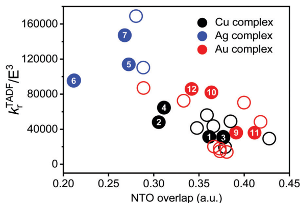
Fig. 7 Relationship between the reduced TADF radiative decay rate versus NTO overlap of the 1 ICT state. The closed symbols are from this work and the open symbols are for previously reported (carbene)M(carbazolyl) complexes. See the ESI† for the identities of the literature complexes.
