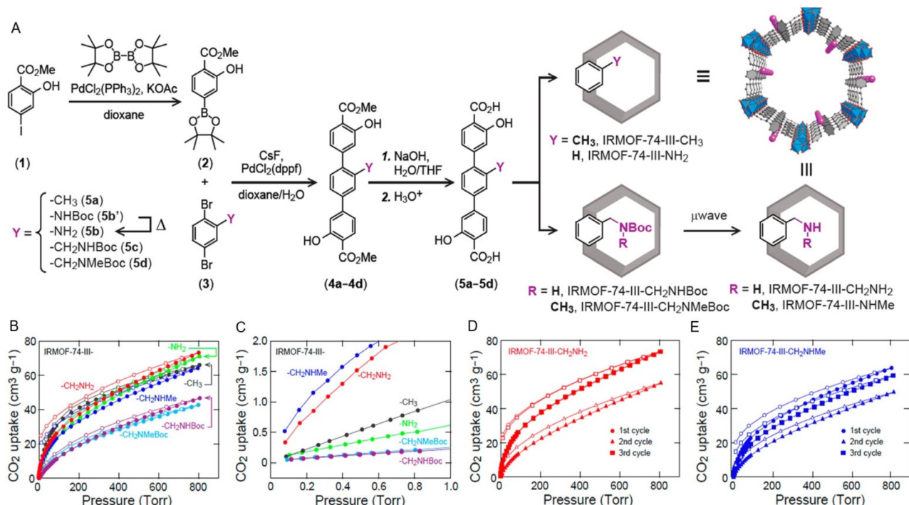
Fig. 7 (A) Synthetic pathway for the functionalized organic linkers used in the synthesis of IRMOF-74-III, in the preparation of -CH 3 (5a), -NH 2 (5b), -CH 2 NHBoc (5c), and -CH 2 NMeBoc (5d) functionalized linkers. On the right is shown a schematic representation of the IRMOF-74-III pore as functionalized with the organic linkers 5a–5d and post-synthetic deprotection of Boc groups. Color code: C in gray, O in red, functional groups in purple, Mg as blue polyhedra. (B) Comparison of CO 2 uptake at 25 °C for IRMOF-74-III-CH 3 (gray), -NH 2 (green), -CH 2 NH 2 (red), -CH 2 NHMe (blue), -CH 2 NHBoc (purple), and -CH 2 NMeBoc (cyan). (C) Expansion of the low-pressure range (>1 Torr). Carbon dioxide isotherms at 25 °C for IRMOF-74-III-CH 2 NH 2 (D) and -CH 2 NHMe (E). Uptakes for samples after activation (first cycle), after first CO 2 uptake (second cycle), and after 120 °C heating for 1 h for regeneration (third cycle) are shown in circles, triangles, and squares, respectively. Reprinted from ref. 36 with permission. Copyright 2014 American Chemical Society.
