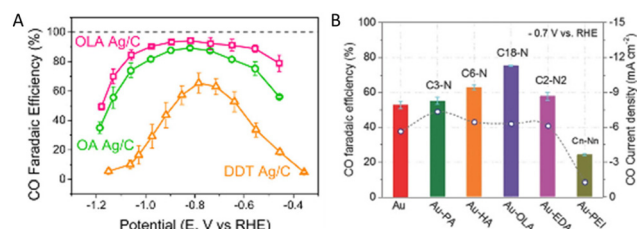
Fig. 21 (A) \text{FE}_{\text{CO}} of OLA-, OA- and DDT-modified Ag NPs supported on carbon black (Ag/C). (B) \text{FE}_{\text{CO}} (column) and CO current density (circle) of different Au catalysts at -0.7 \text{ V} (vs. RHE). Adapted from ref. 183 and 182 with permission. Copyright 2017 American Chemical Society and 2018 Wiley-VCH.
