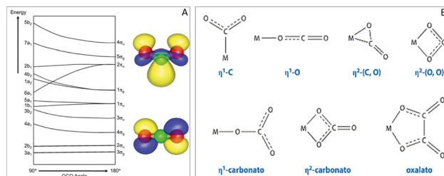
Fig. 8 (A) Walsh diagram of CO 2 , with illustrations of the highest occupied molecular orbitals of the anion (top) and the neutral (bottom). (B) Structural motifs of metal–CO 2 interactions. Reprinted from ref. 43 and 44 with permission. Copyright 2014 Abingdon: Taylor & Francis and 2018 Annual Reviews.
