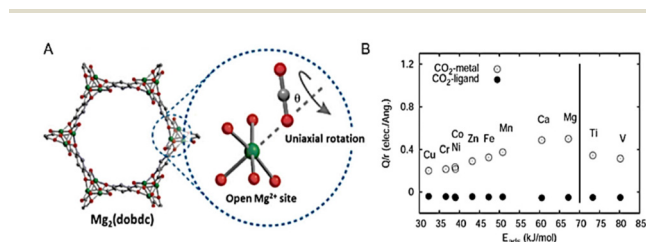
Fig. 6 (A) Schematic illustration of \text{CO}_2 uniaxial rotation at the open \text{Mg}^{2+} site in \text{Mg}_2(\text{dobdc}) . Gray – C, red – O, and green – Mg atoms; H atoms are omitted for clarity. The blue circle is the arbitrary rotation axis. (B) \text{CO}_2 adsorption energy plotted over Q/r computed for the metal– \text{CO}_2 oxygen distance and the tetrazole nitrogen– \text{CO}_2 carbon distance. The vertical line is to guide the eye. Reprinted from ref. 33 and 34 with permission. Copyright 2012 and 2014 American Chemical Society.
