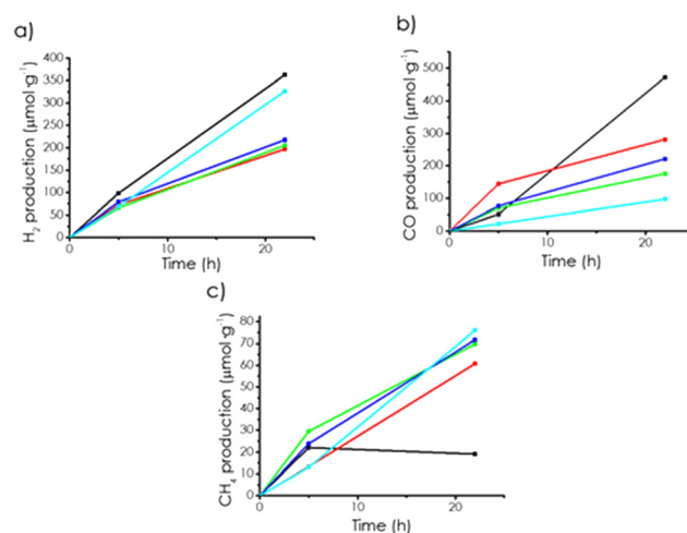
Fig. 4 Temporal profiles of (a) H 2 , (b) CO, and (c) CH 4 evolution for mp-C α (black), mp-C β (red), mp-C γ (green), mp(N)-C α (blue), and mp(P)-C α (cyan) upon the irradiation of CO 2 dissolved in CH 3 CN/H 2 O containing TEOA with the output of a 300 W Xe lamp.
