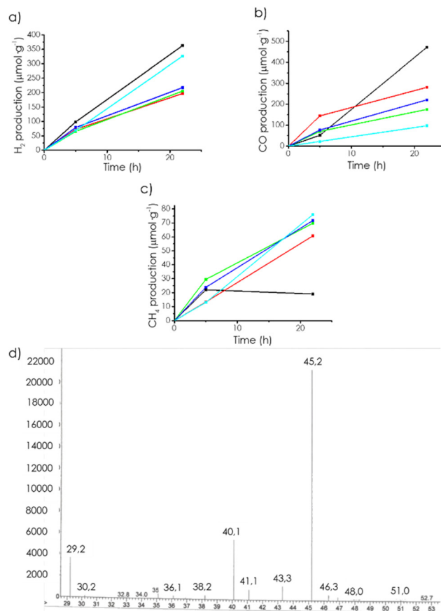
Fig. 3 Temporal gas evolution from CO 2 dissolved in a CH 3 CN/H 2 O mixture containing TEOA using mp-C α (black), mp-C β (red), mp-C γ (green), mp(N)-C α (blue), and mp(P)-C α (cyan) as photocatalysts upon 300 W Xe lamp irradiation: (a) H 2 , (b) CO, (c) CH 4 , (d) mass spectra of the test using 13 CO 2 as the substrate and mp-C α as the photocatalyst.
