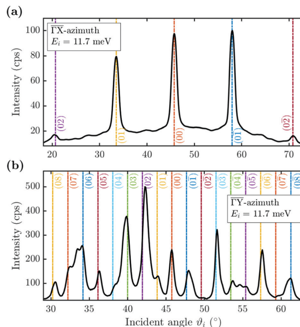
Fig. 2 Diffraction scans along the two high-symmetry directions upon scattering parallel ( \overline{\Gamma}\overline{X} (a)) and normal ( \overline{\Gamma}\overline{Y} (b)) to the steps, plotted versus incident angle \vartheta_i at a sample temperature of T_s = 113 K. The individual diffraction peaks are labelled with the interacting \mathbf{G} -vector.
