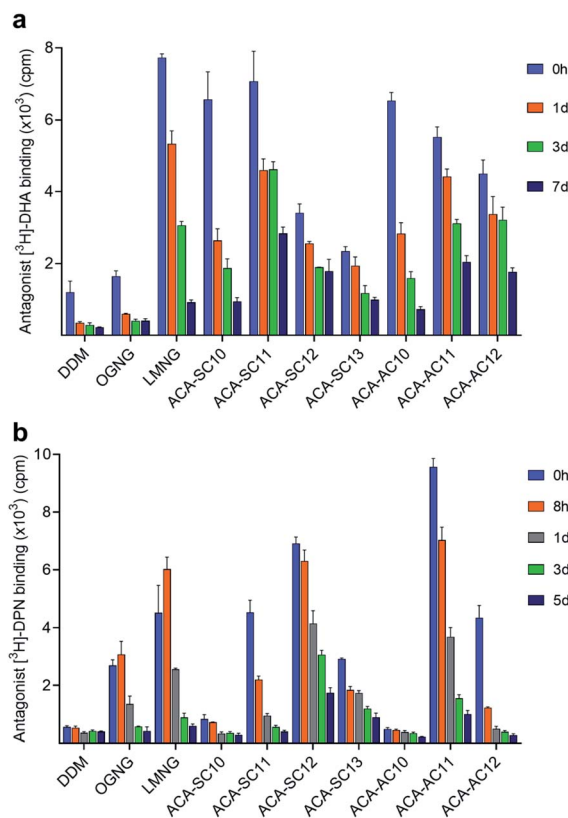
Fig. 5 Evaluation of the new detergent for (a) \beta_2 AR and (b) MOR stability. DDM , OGNG and LMNG were used as control agents. \beta_2 AR and MOR purified in DDM and LMNG , respectively, were diluted into a buffer containing the indicated detergents to reach final detergent concentrations of 0.2 and 0.1 wt%. The receptor ability to specifically bind a radioactive antagonist ( [^3H] -dihydroalprenolol (DHA) ( \beta_2 AR) or [^3H] -diprenorphine (DPN) (MOR)) was monitored at regular intervals during a 7 day incubation at room temperature ( \beta_2 AR) or a 5 day incubation at 4 °C (MOR). Data points are mean \pm SEM (error bars); n = 3 .
