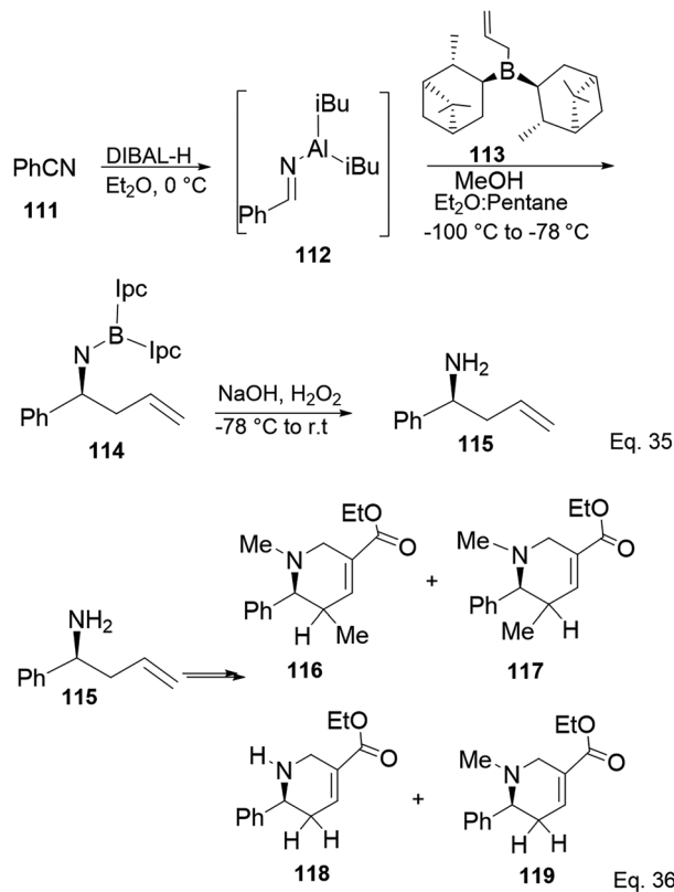
Fig. 11 Pinene-derived iminodiacetic acid (PIDA).
