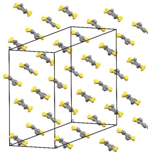
Fig. 2 Packing arrangement of the donor layer for 4. Salts 1–4 are isostructural. Hydrogen atoms and minor disorder components are omitted for clarity.
