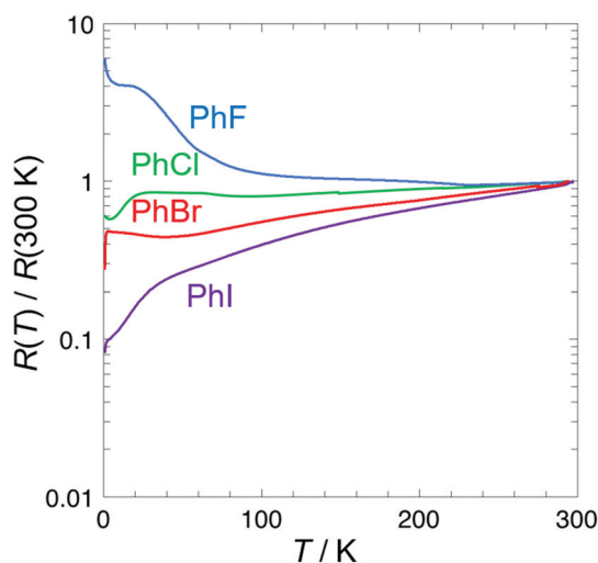
Fig. 6 Electrical resistivity for salts 1–4 .
