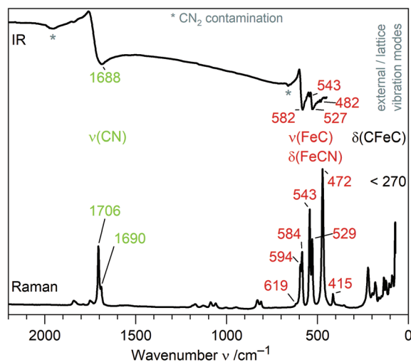
Fig. 2 IR and Raman spectra of (\text{Sr}_3\text{N})_2[\text{Fe}(\text{CN})_4] with assigned molecular vibrations of [\text{Fe}(\text{CN})_4]^{6-} .
