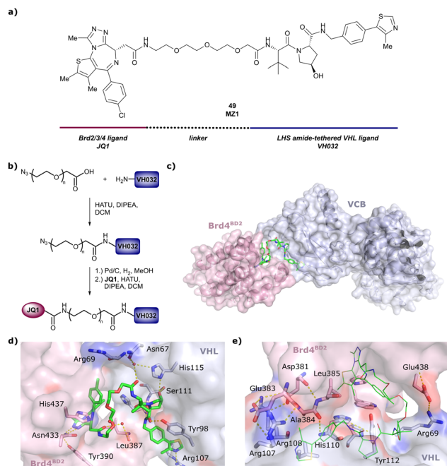
Fig. 17 Development of first VHL targeting PROTAC degrader. Structure of MZ1 ( 49 ) (a), synthetic route to access such degraders (b), and ternary cocystal structure of MZ1 bound to VCB and Brd4 BD2 (c), PROTAC–protein interactions (d) and de novo PPI between Brd4 BD2 and VHL (e) (PDB 5T35). 102
