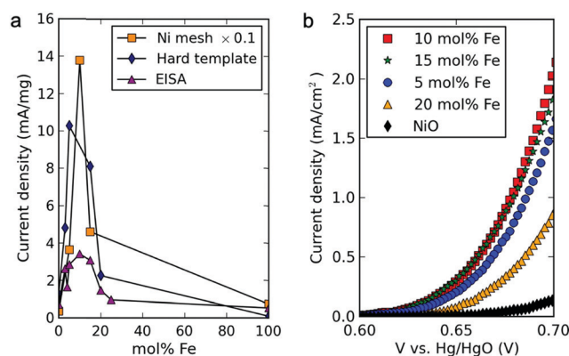
Fig. 37 (a) Electrochemical oxygen evolution activity at a fixed over-potential of 360 mV for the varying synthesis methods and compositions of mixed metal oxide electrocatalysts. (b) Geometric area-normalised polarisation (scan rate = 1 \text{ mV s}^{-1} ) data of mixed Ni–Fe oxide catalysts (synthesised by the EISA method) showing the highest activity for 10 mol % Fe oxide. Reproduced with permission from ref. 736 Copyright American Chemical Society 2012.
