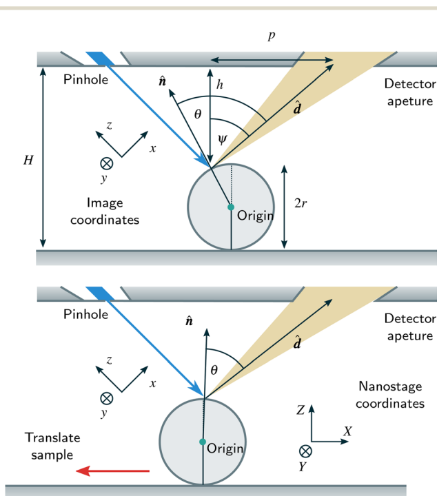
Fig. 7 Co-ordinate system and vectors used in the derivation of the relation between image positions and incidence and detection angles. \hat{d} is the vector towards the detector, and \hat{n} is the unit normal to the sphere at the beam-sphere intersection point. The coordinate system is defined to have the z axis parallel to the beam and the origin at the centre of the sphere. The distance from the scattering point to the pinhole plate h does vary across the sphere but can be neglected for small enough spheres.
